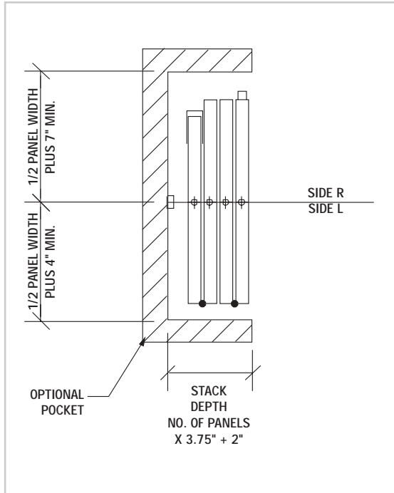
Expandable Jamb Closure - Even Panel Quantity
