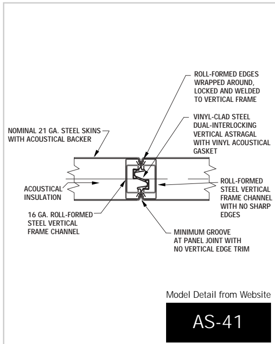
Standard Panel Joint
