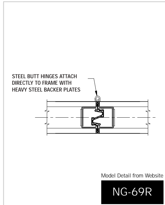
Standard Hinged Panel Joint
