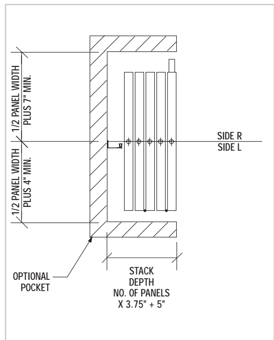
Angle Jamb Closure - Odd Panel Quantity
