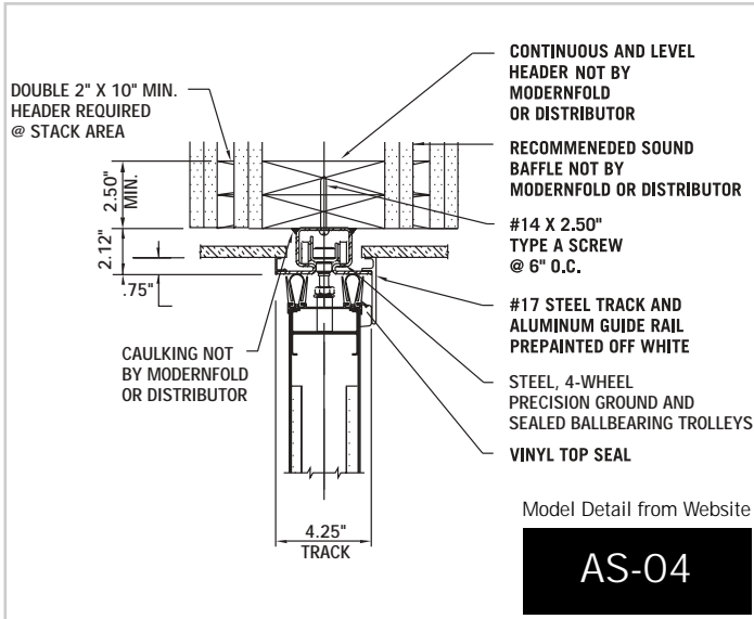
#17 Track System Direct Mount
