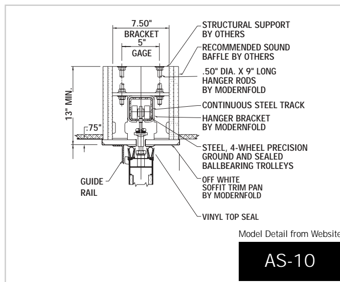
#14 Track System Bracket Mount
