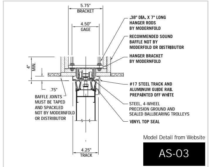
#17 Track System Bracket Mount
