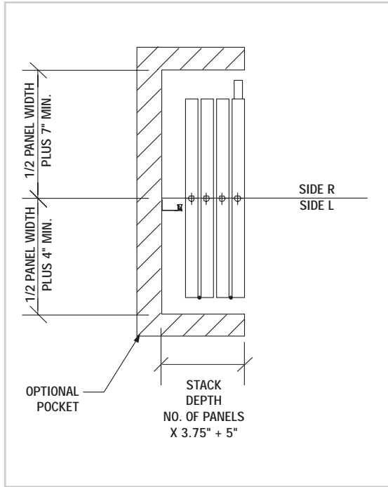
Angle Jamb Closure - Even Panel Quantity
