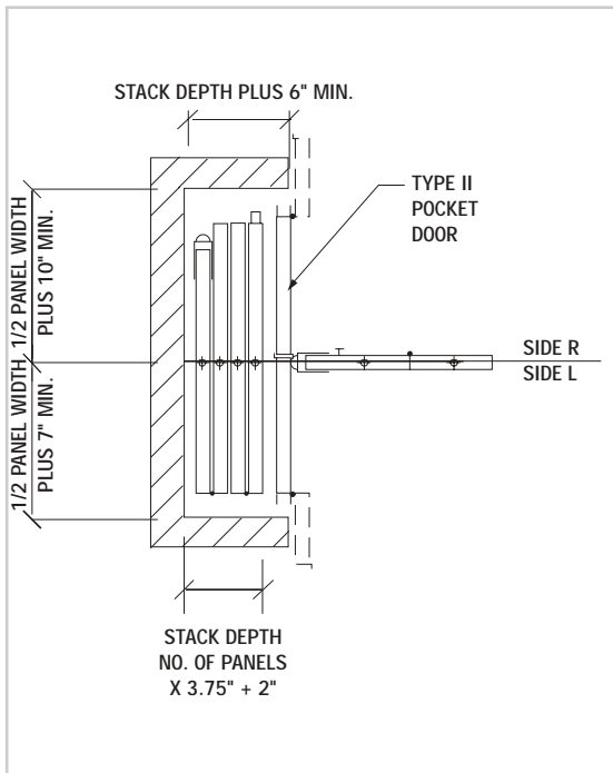
Remote Expandable Jamb Closure
