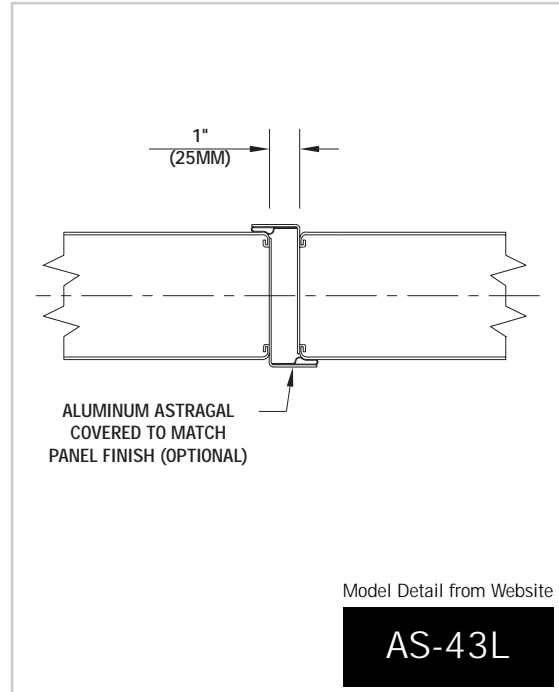
Hinged Panel Meeting w/ Pass Door Astragal
