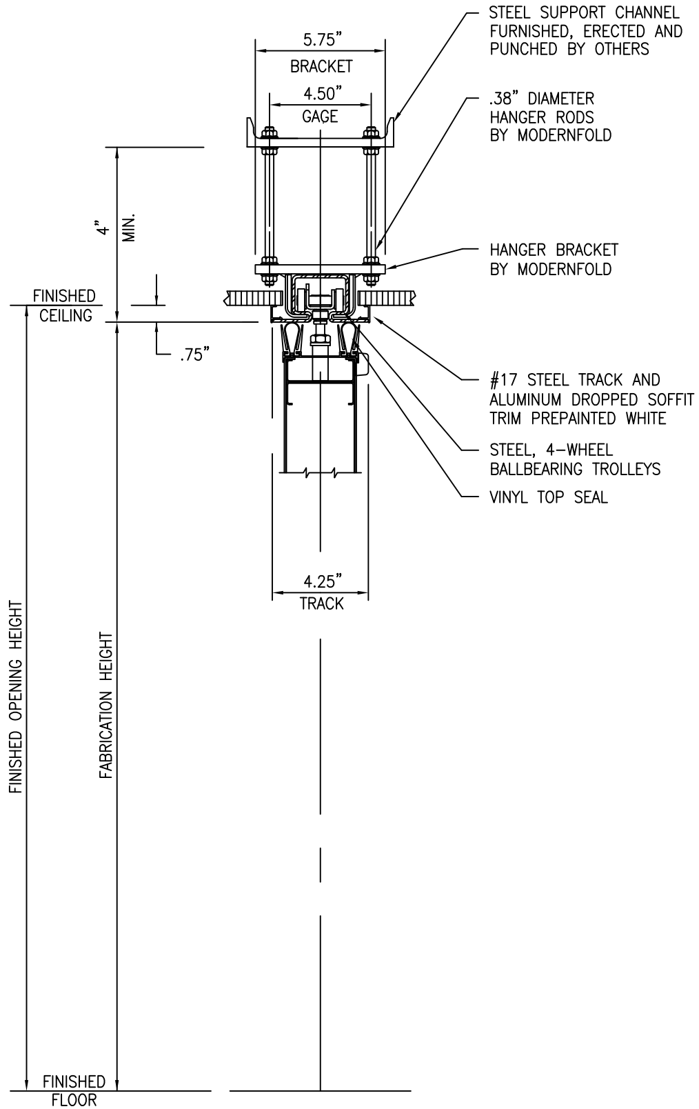
#17 TRACK / STANDARD BRACKETS / NO GUIDERAIL / STEEL CHANNEL
