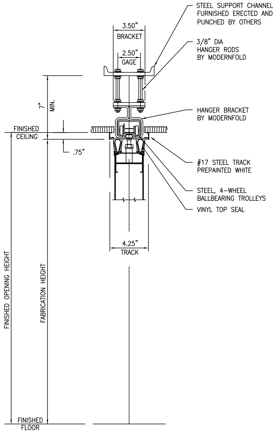
#17 TRACK / HEAVY DUTY (2.5 GUAGE) BRACKETS / STEEL CHANNEL
